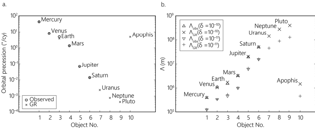
Figure 1. Comparison between the observed orbital precession of the selected Solar System bodies and the corresponding GR predictions (a); Constraints on range of interaction \Lambda in the case of \delta = 10^{-11} and 10^{-10} , obtained from the observed orbital precession and its GR prediction (b).
