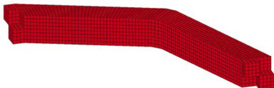
Figure 8. Meshing of one connection in the simulation procedure.
