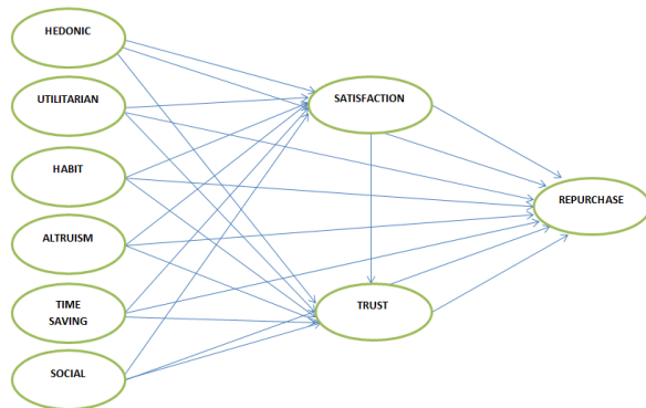
Figure 3. Theoretical Model
