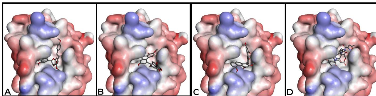
Figure 1. Visualization of strongest conformation secondary metabolites of Dendrobium spp., with M pro A. Dendrocandin, B. Denthyrsinone, C. Denthyrsinol, D. Inhibitor N3
