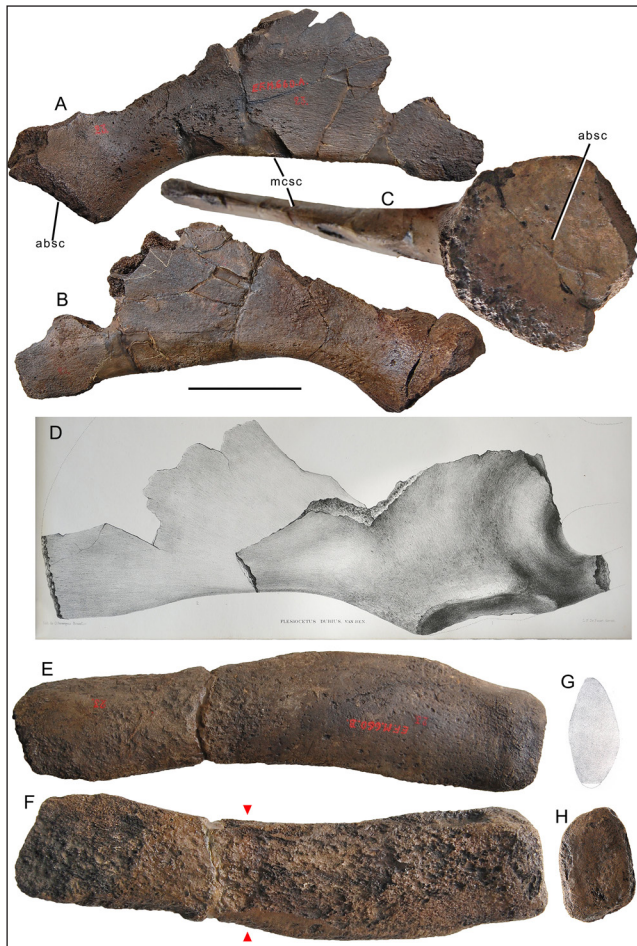
Fig. 10 - Specimen M. 660. A) specimen M. 660a, right scapula in lateral view; B) the same in medial view; C) the same in ventral view; D) the same in lateral view from Van Beneden (1885). E) specimen M. 660b, left radius in lateral view; F) the same in medial view; G) section at the level of the red triangles in F from Van Beneden (1885); H) inferior view of proximal epiphysis. Scale bar equals 10 cm. See Anatomical abbreviations for explanation of acronyms.
