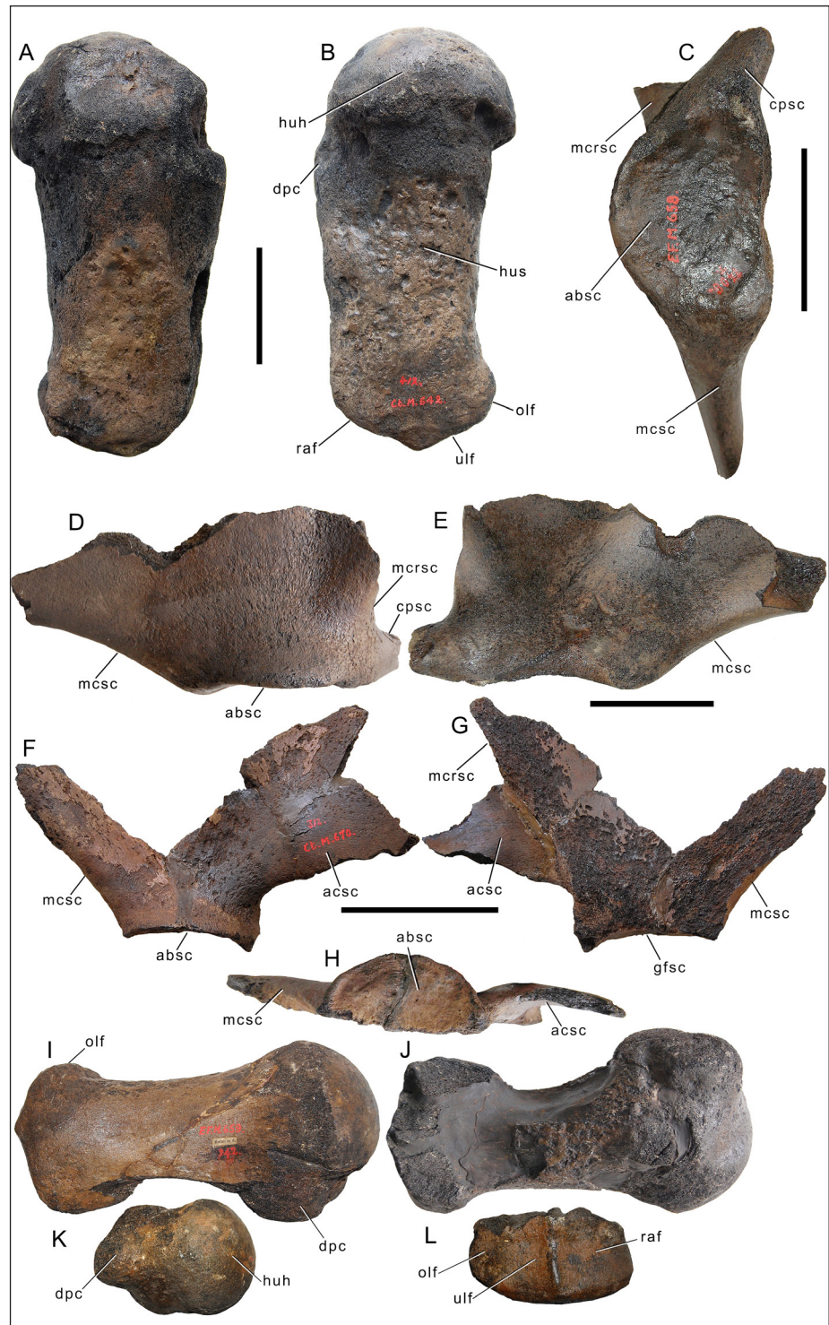
Fig. 17 - Specimen M. 642, left humerus: A) lateral view; B) medial view. Specimen M. 658, right scapula: C) ventral view showing the acetabular fossa; D) lateral view; E) medial view. Specimen M. 670, right scapula: F) lateral view; G) medial view; H) ventral view. Specimen M. 659, humerus: I) lateral view; J) medial view; K) superior view; L) inferior view. See Anatomical abbreviations for explanation of acronyms.
