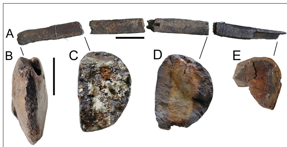
Fig. 22 - Balaenopteridae gen. et sp. indet. Specimen M. 634, right mandibular ramus: A) the four segments forming the ramus in medial view; B) natural cross-section of anterior end of anterior-most segment; C) natural cross-section of posterior end of anterior-most segment; D) natural cross-section of posterior end of penultimate segment; E) natural cross-section of posterior end of posterior-most segment. In A, scale bar equals 10 cm and 5 cm in B.
