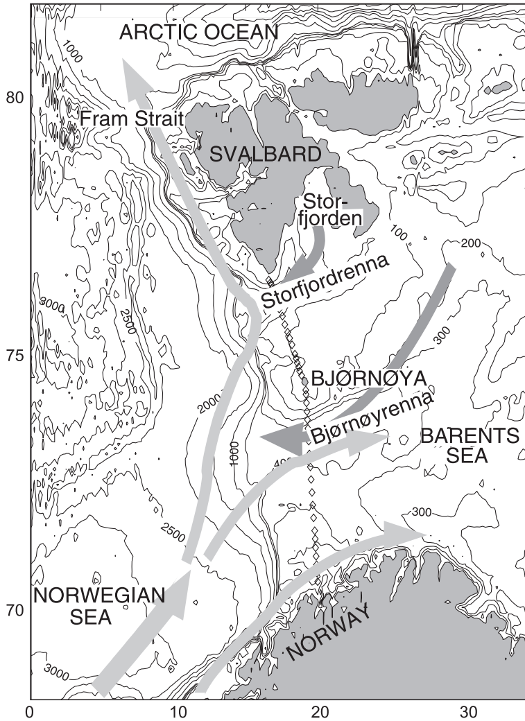
Fig. 1. The main features of the topography and circulation in the BSO. CTD stations are marked ◊.
