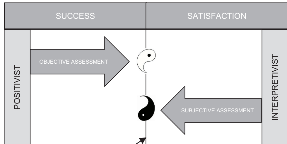
Figure 3 Yinyang framework
