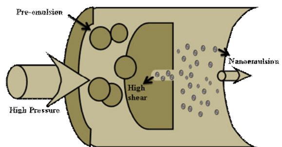
Figure 4. Working principle of ultrasonic emulsifier [1]
