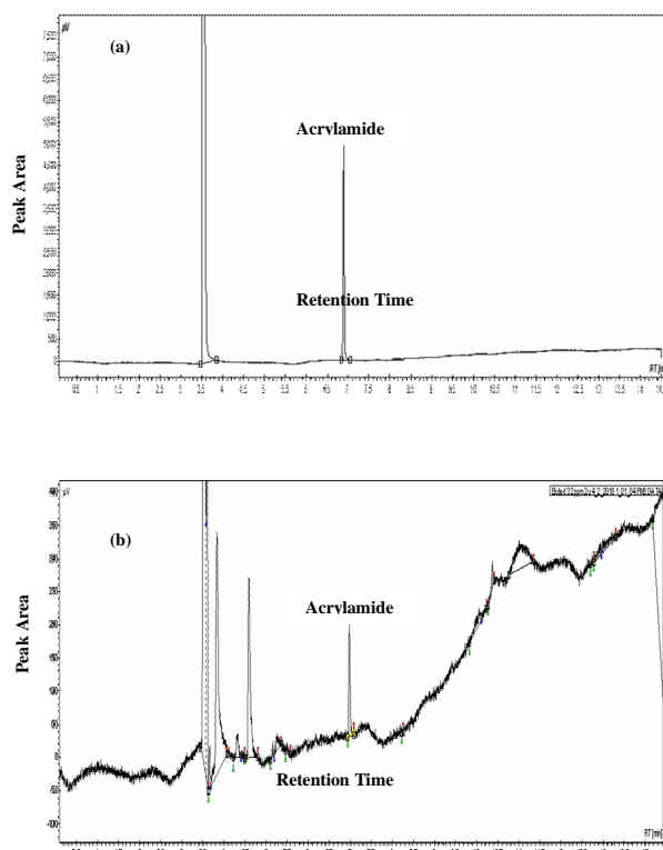
Figure 6. (a) Standard and (b) Acrylamide Standard (5ppm)
