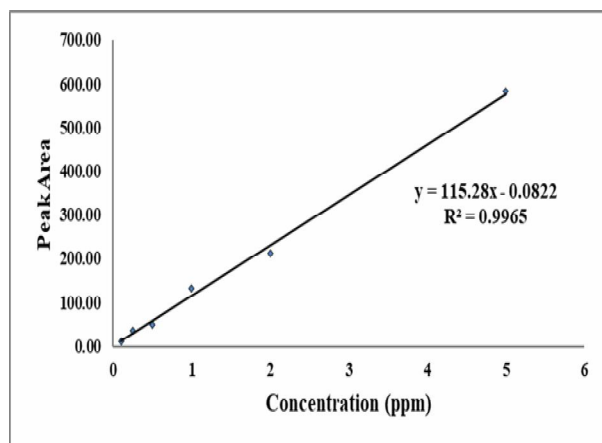
Figure 5. Linearity of Acrylamide determination in spiked potato chips
