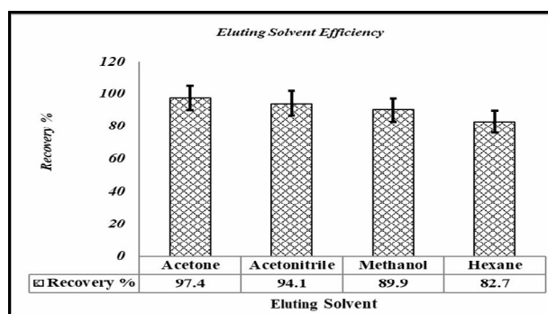
Figure 4. Eluting solvents efficiency. (Acrylamide standard 20 ppm, activated charcoal mass = 400 mg, flow rate = 3 mL/min, 2 \mu L of eluent was injected to GC/NPD)
