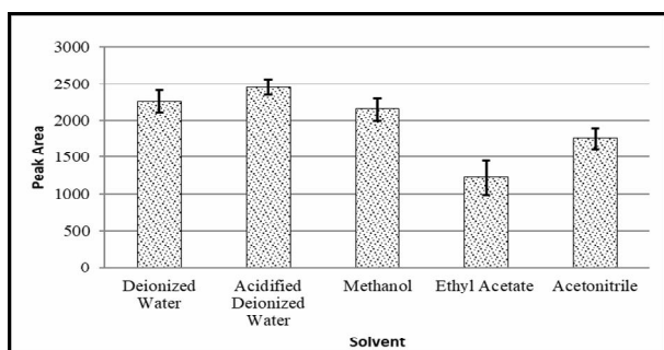
Figure 2. Efficiency of the Extracting Solvents
