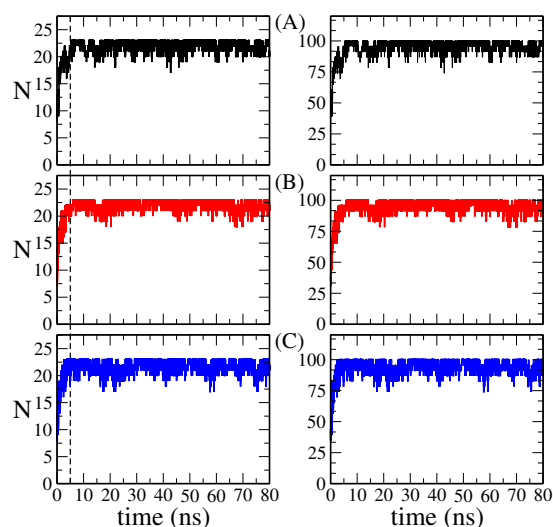
Figure 9: Left column represents the number of calcium ions involved in the lipid coordination along time for a concentration of [CaCl_2] = 0.25 N at different temperatures: (A) T = 330 K, (B) T = 340 K and (C) T = 350 K. The right column shows the same information expressed as a percentage of the total number of calcium ions in solution.
