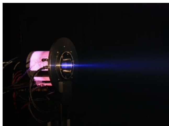
Figure 5: RIT10/37 thruster in operation in the STG-ET.
