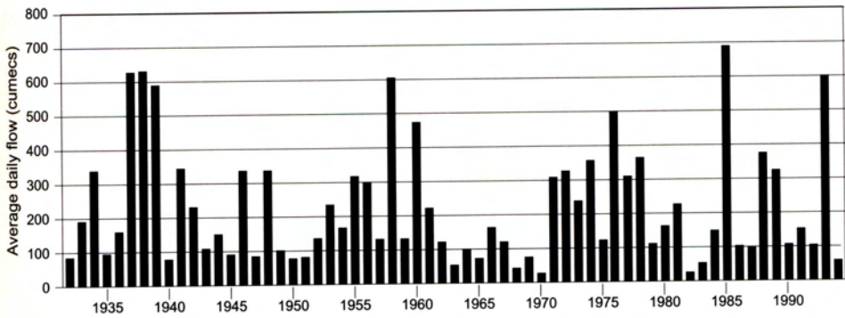
Fig. 6. Simulated peak annual flows for the Sabie River at section 4 based on the ACRU hydrologic model.
