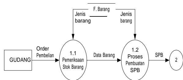
Figure 4.13 Process 1 Level 1 Diagram
