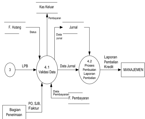
Figure 4.16 Level 1 Process Diagram 4
