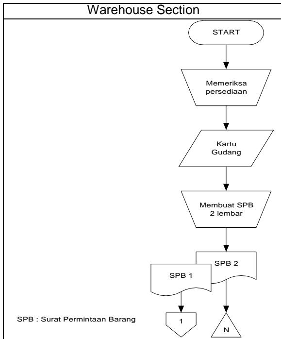
Figure 4.1 Credit Purchase Procedures in the Warehouse Section
