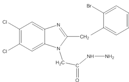
Scheme 1. Chemical structure of DIBBA.
