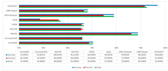
Figure 2. Comparison of the Average Values of Accuracy, Precision, and Recall of the k-NN Algorithm on Various IDS Datasets
