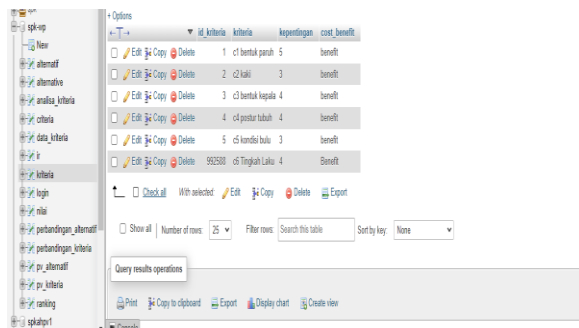
Figure 5. Database View
