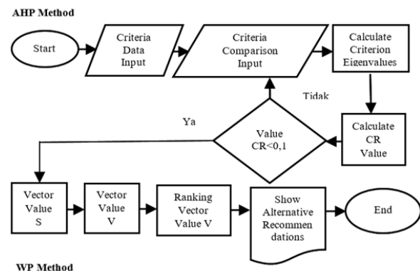
Figure 3. Flowchart System
