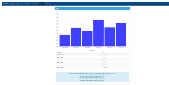
Figure 10. Analysis View
