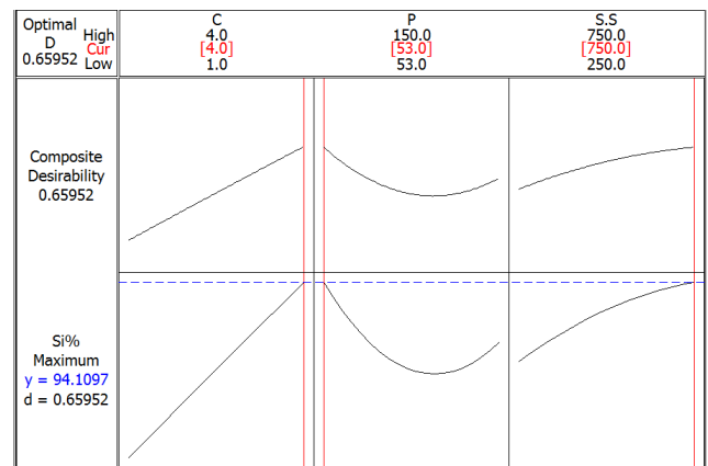
Figure 4. Optimization chart for maximum of recovery Si element.
