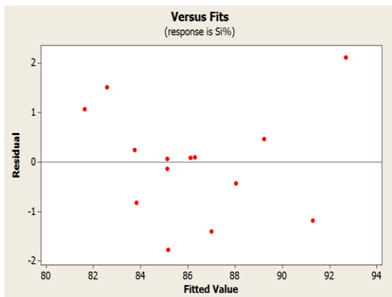
Figure 3. Plot of residuals vs value of recovery Si element
