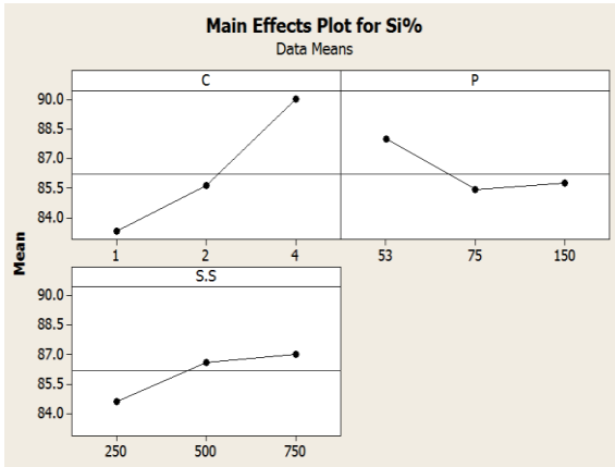
Figure 1. Main effect plot of residuals of recovery Si element
