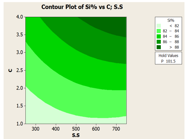
Figure 5. Three-dimensions and contour plots of recovery Si.
