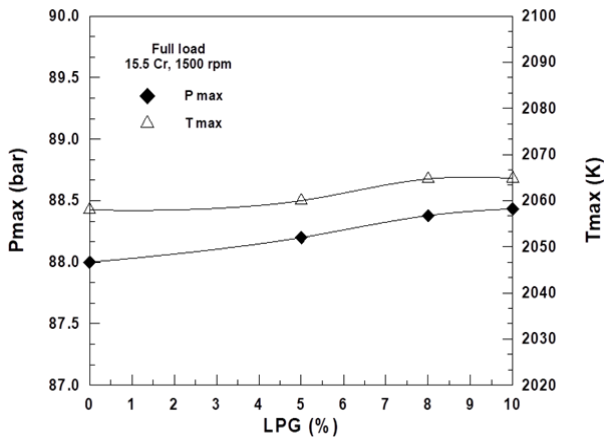
Figure 6. effect of varying LPG on the maximum (pressure and temp.)
