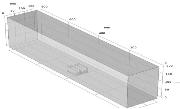
Figure 2. 3D computational domain the wind channel
