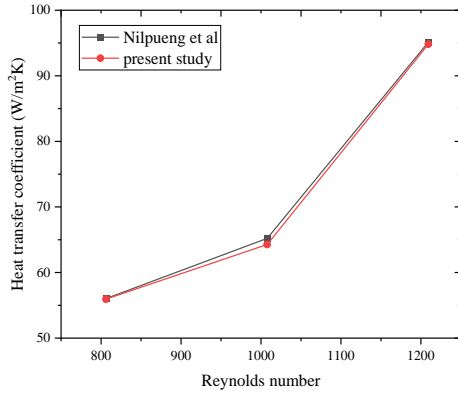
Figure 4 Comparison the heat transfer coefficient versus Re between the current work with those obtained by Nilpueng et al[1] at , q= 14.81kW/m 2
