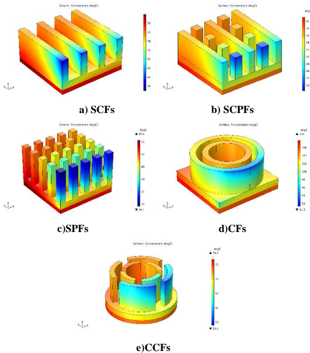
Figure 5. Surface temperature gradients for all heat sink geometries at velocity 2.4 m/s, Pin= 40W
