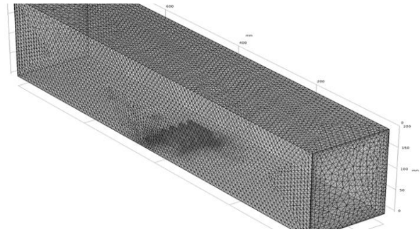
Figure 3. 3D computational quadratic mesh of the domain
