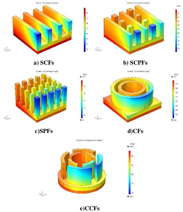
Figure 6. Surface temperature gradients for all heat sink geometries at velocity 1.8m/s, Pin = 40W
