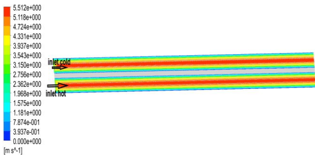
Figure .6 contour explains the distribution of velocity (m/sec) at PFMCHC on (y-z) plane at D_h=10 \mu\text{m} and Re=30 .
