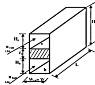
Figure . 2 A unit of heat exchange consists of the hot and cold channel [14].
