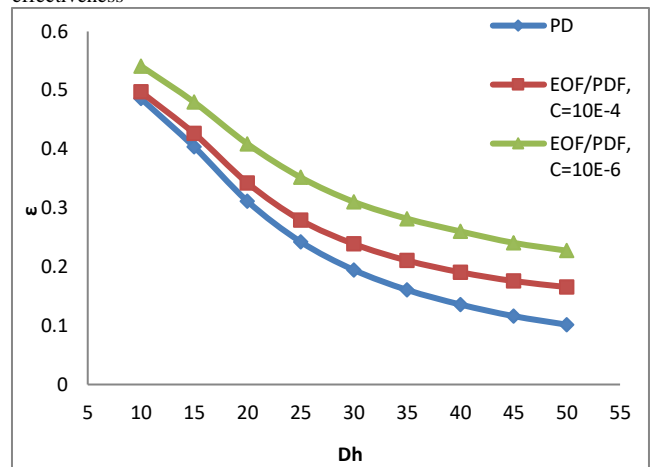
Figure .12 Variation of effectiveness with a hydraulic diameter (μm).
