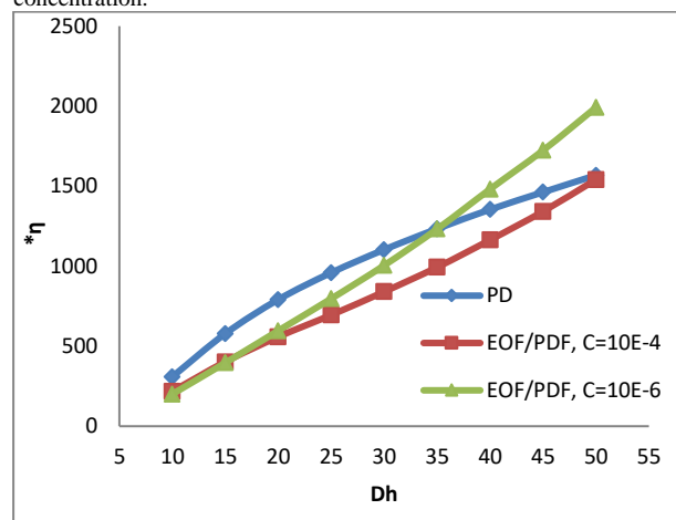
Figure .16 variation of overall performance with a hydraulic diameter
