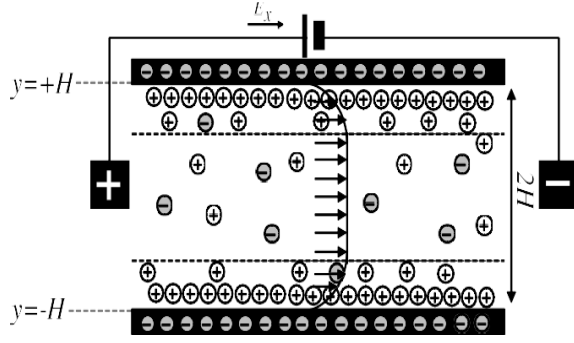
Figure . 3 Scheme formed of electric of double layer on the surface wall [16]
