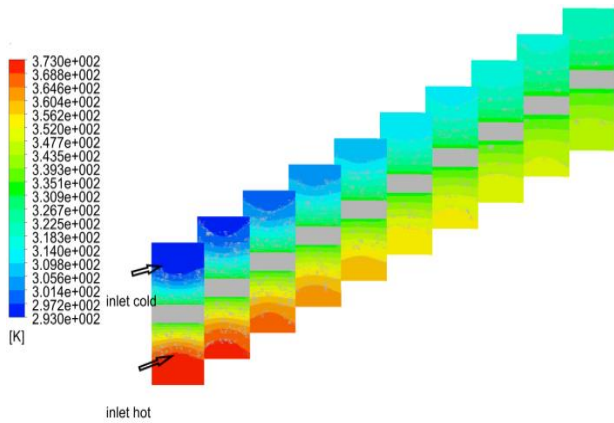
Figure .9 contour of temperature distribution (K) for many planes of parallel flow MCHE Dh=10 μm and Re =50.
