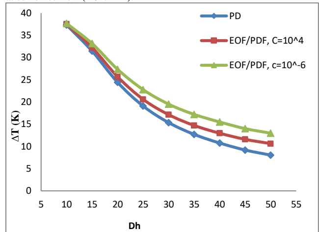
Figure .11 variation of average temperature difference with the hydraulic diameter (μm).
