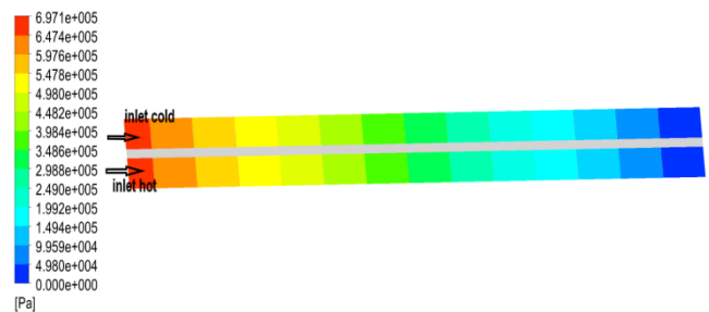
Figure .8 contour pressure distribution along the cold channel and hot channel of parallel flow MCHE for D_h=10 \mu\text{m} and Re=30 .
