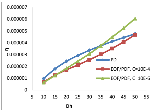
Figure. 13 Variation of overall performance with a hydraulic diameter(μm).
