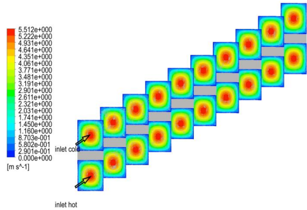
Figure .7 contour represents the variation of velocity (m/s) along the hot and cold channels at parallel flow MCHE, D_h=10 \mu\text{m} , and Re=30 .
