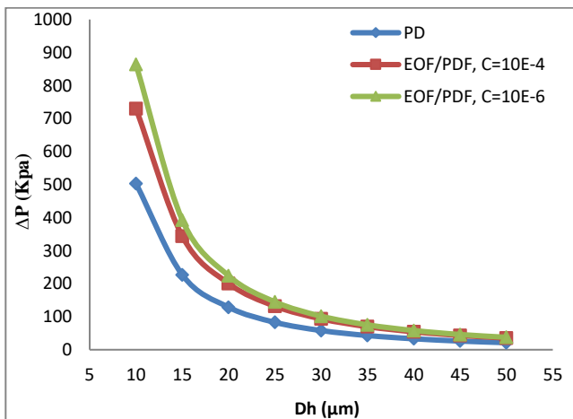
Figure. 10 variation of total pressure drop (KPa) with a hydraulic diameter (μm).
