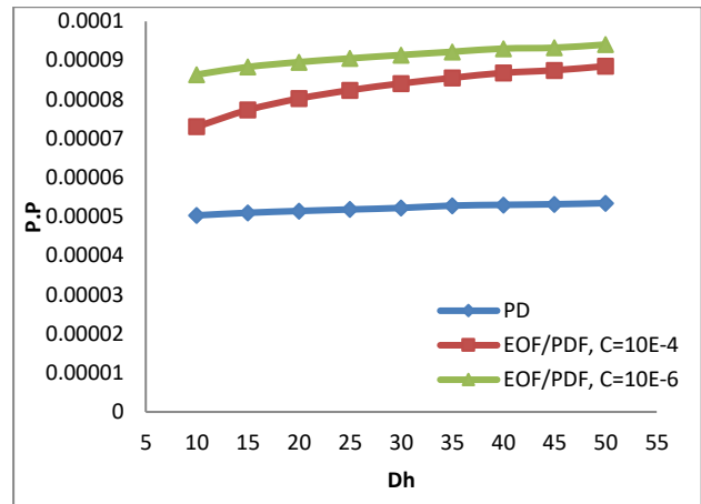
Figure .15 variation of pumping power (watt) with a hydraulic diameter.
