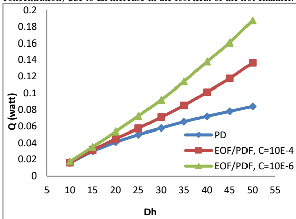
Figure .14 variation of average heat transfer (watt) with a hydraulic diameter
