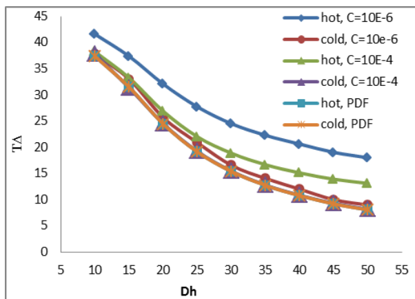
Figure .17 variation of temperature different for hot and cold channel with a hydraulic diameter ( \mu\text{m} ).
