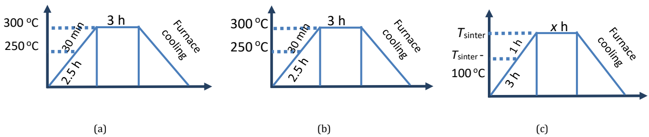
Fig. 8. Heating condition of (a) pre-fire process of \text{La}_2\text{O}_3 (b) calcination process (c) sintering process
