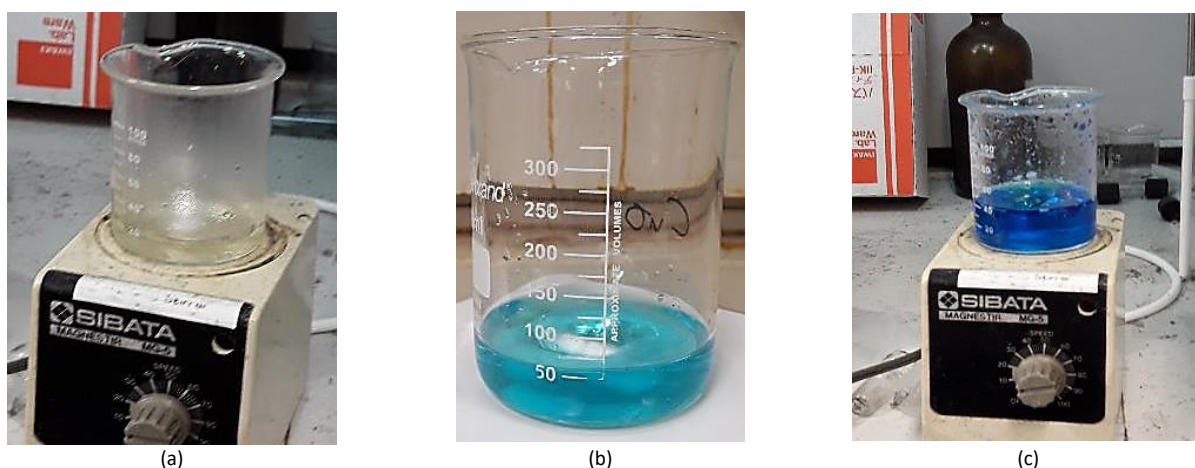
Fig. 1. The photograph of (a) La(NO_3)_3 \cdot 6H_2O solution (b) Cu(NO_3)_2 solution (c) Homogeneous solution of La(NO_3)_3 \cdot 6H_2O , Cu(NO_3)_2 , citric acid, and ethylene glycol.
