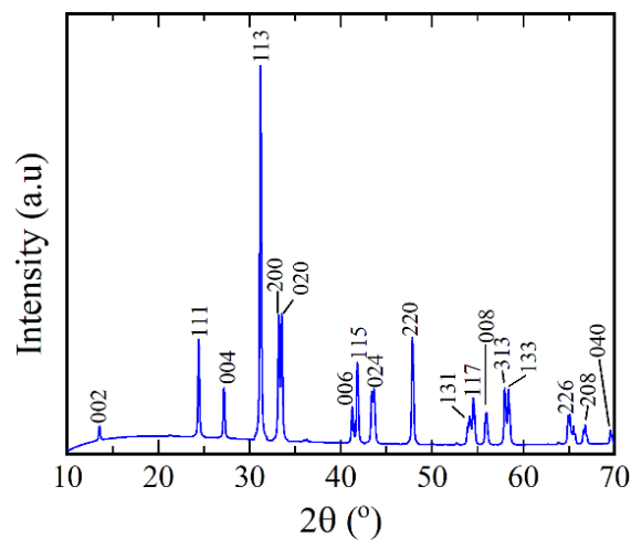
Fig. 9. XRD pattern of \text{La}_2\text{CuO}_4 nanoparticles prepared by sol-gel method.
