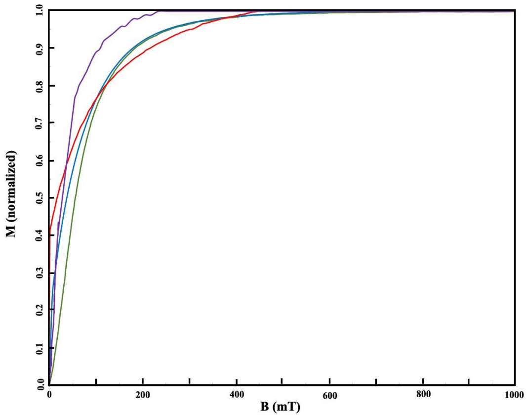
Fig. 1. The typical digitized IRM acquisition curves used in this study. Red curve represents volcanic lavas (IJ-1), green curve represents volcanic ashes (Bromo), blue curve represents lake sediments (TOW9-4-125), and purple curve represents fly-ash (KTPS ASH)
