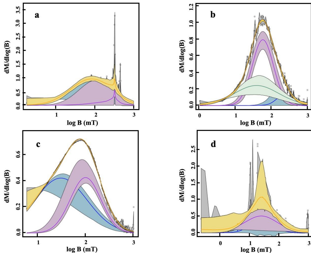
Fig. 3. Coercivity models issued by MAX Unmix after adjustment or curve-fitting process. (a) volcanic lavas (IJ-1), (b) volcanic ashes (Bromo), (c) lake sediments (TOW9-4-125) and (d) fly-ash (KTPS ASH). Blue lines represent the first coercivity component, purple lines the second coercivity component, and green lines the third coercivity component. The yellow lines represent the best-fit coercivity model or spectrum based on the data shown in grey lines. All data, except for the fly ash show good fit between the model and the data. See text for explanation.
