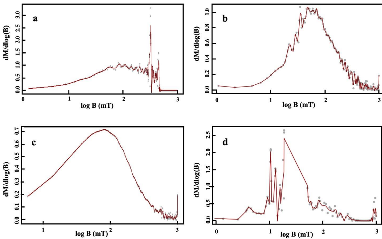
Fig. 2. The typical raw coercivity spectrum issued by MAX Unmix prior to adjustment or curve-fitting process. (a). volcanic lavas (IJ-1), (b) volcanic ashes (Bromo), (c) lake sediments (TOW9-4-125) and (d) fly-ash (KTPS ASH)
