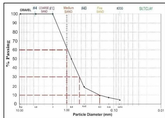
Fig. 2. Graph Sieve analysis on Drill Sample 1 (4.50-5.00) M.
