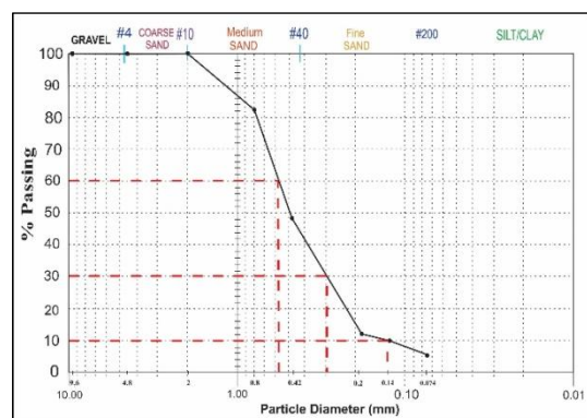
Fig. 4. Graph Sieve analysis on Drill Sample 3 (8.00-8.50) M.
