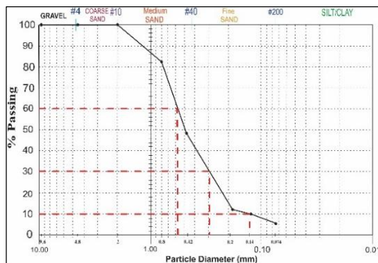
Fig. 3. Graph Sieve analysis on Drill Sample 1 (8.00-8.50) M.
