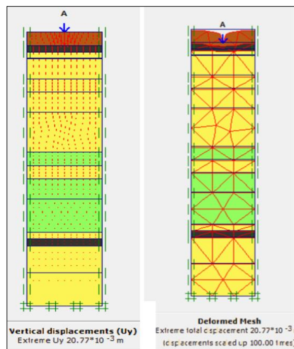
Fig. 6. Plaxis Modeling On Declining Soil.
