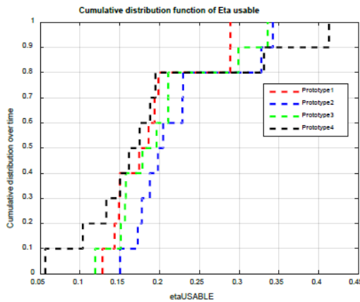
FIG. 13 \eta_{usable} cumulative frequency distribution for Adaptiwall prototypes
