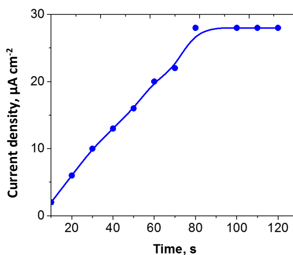
Figure 7. Effect of accumulation time on the AdSV response of dinoterbon at NiO-GO/GCE; rest time: 10 s; stirring rate: 1500 rpm; scan rate: 20 mVs -1 ; concentration: 5.0 µg mL -1 ; pH: 4.0 (BR buffer); pulse amplitude: 25mV.
