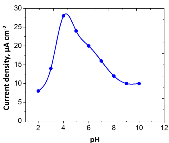
Figure 6. Effect of pH on dinoterbon at NiO-GCE/GCE; accumulation time: 80 s.; rest time: 10 s.; stirring rate: 1500 rpm; scan rate: 20 mVs -1 ; concentration: 5.0 µg mL -1 ; pulse amplitude: 25 mV.
