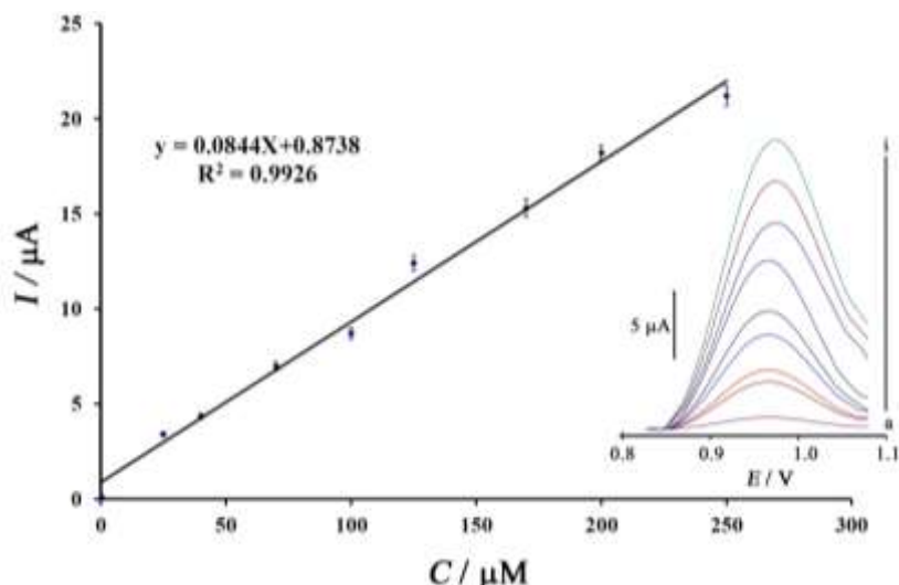
Figure 4. Current – concentration curve for monitoring of lorazepam using HMIImCl/ZnO-NPs/PE. Inset) Square wave voltammograms of lorazepam at surface of HMIImCl/ZnO-NPs/PE in the concentration of 1) 0.5; 2) 25; 3) 40; 4) 70; 5) 100; 6) 125; 7) 170; 8) 200 and 9) 250 \mu\text{M} ( n=4 )
