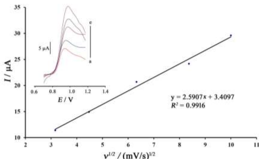
Figure 3. Current vs. v^{1/2} plot for oxidation of 300 \mu\text{M} lorazepam at surface of HMIImCl/ZnO-NPs/PE. Linear sweep voltammograms of 300 \mu\text{M} lorazepam at scan rates; a) 10; b) 20; c) 40; d) 70 and e) 100 mV/s ( n=4 )
