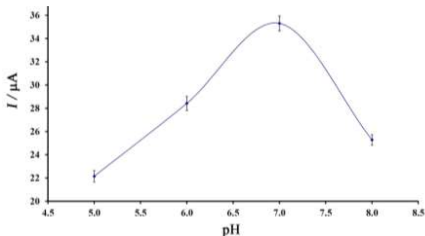
Figure 1. Current-pH diagram for sensing of 300 \mu\text{M} lorazepam using HMImCl/ZnO-NPs/PE as electroanalytical sensor ( n=4 )
