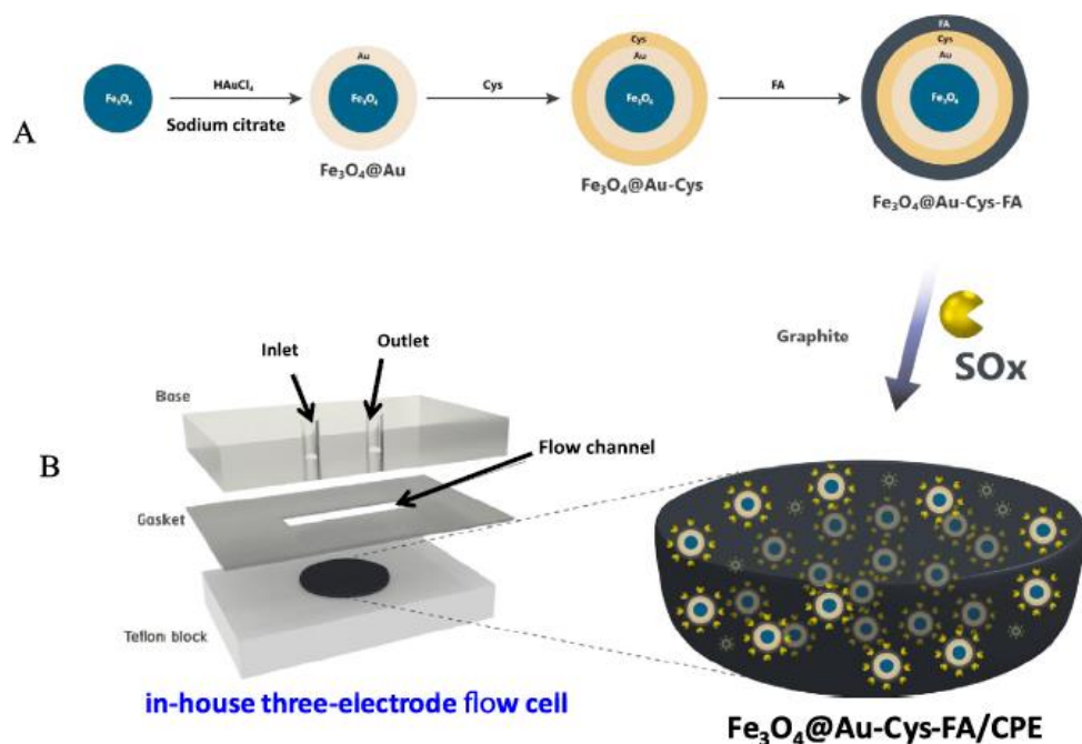
Figure 3. Preparation process of the sulfite bio-sensors (A) \text{Fe}_3\text{O}_4\text{@Au-Cys-FA} nano-composite with the immobilized \text{SO}_x^- ; (B) \text{Fe}_3\text{O}_4\text{@Au-Cys-FA} modified CPE [157]
