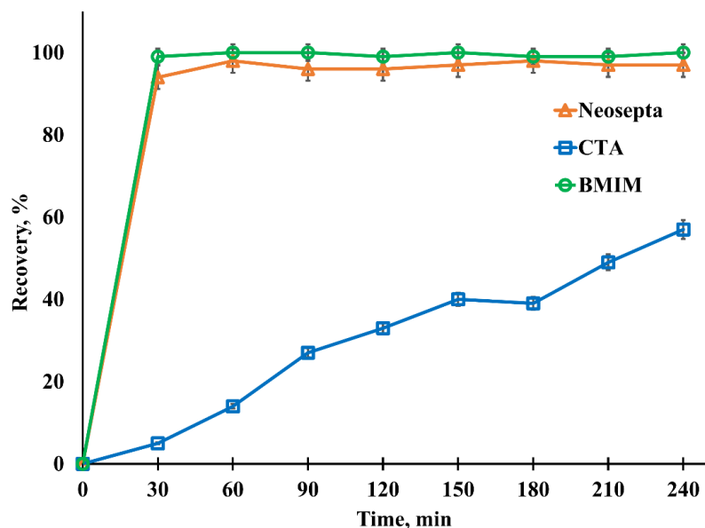
Figure 7. Influence of different types of the membrane towards the recovery of 100 mg/L of \text{Pd}^{2+} in 0.2 M NaCl
