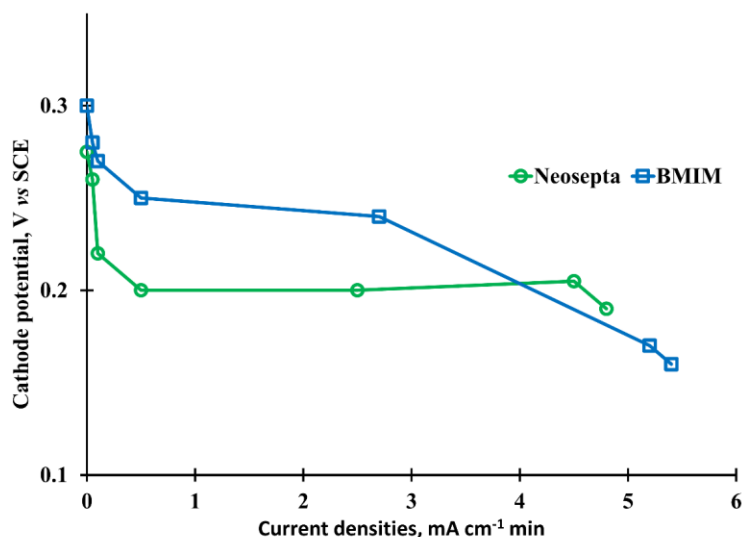
Figure 8. Polarization curves of RVC cathode using different types of ion exchange membrane
