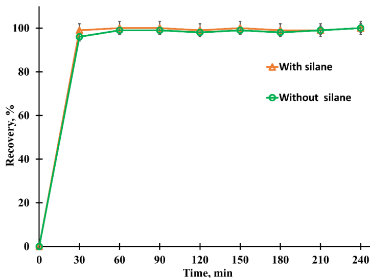
Figure 6. Effect of silane in PIM on recovery of 100 mg/L of \text{Pd}^{2+} in 0.2 M NaCl. PIM composition: 0.1 g CTA, 0.08 g BMIM-Cl, 0.03 g silane
