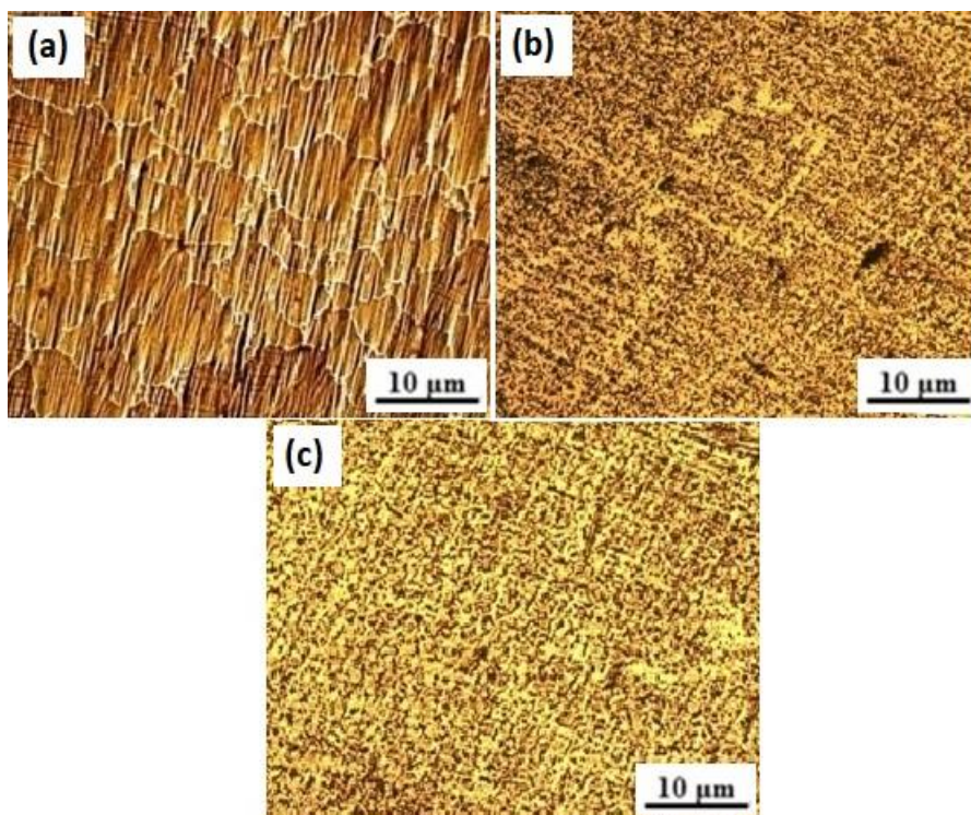
Figure 6. OM image showing the microstructural features in (a) PM, (b) FSPed, and (c) NMMSCs specimens
