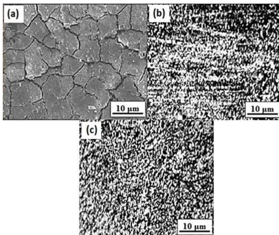
Figure 8. SEM image representing the microstructural features in (a) PM, (b) FSPed, and (c) NMMSC specimens
