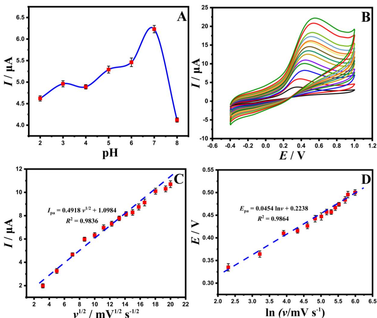
Figure 5. A - The I pa vs. pH curve for electro-oxidation of AA at the surface of L-cys@MAPbI 3 /GCE; B - CVs of L-cys@MAPbI 3 /GCE in the presence of 0.1 M KCl containing 1.0 μM AA; C - The plot of I pa against v 1/2 relative to electro-oxidation of 1.0 μM AA at L-cys@MAPbI 3 /GCE; D - The plot of E pa vs. natural logarithm
