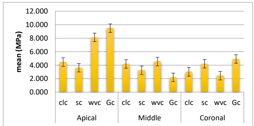
Figure (2): The average bond strength values ( in MPa).
