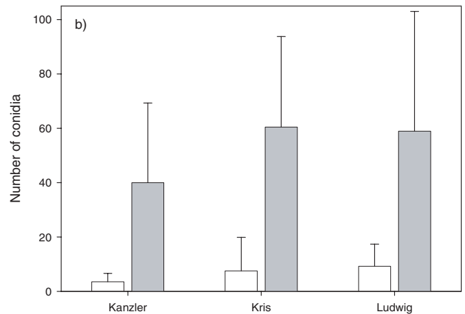
Fig. 4: Number of conidia remaining on the surfaces of three wheat cultivars with intact (open bars) and wiped (filled bars) wax crystals after inoculation and rain treatment. Intervals between inoculation and rain treatment: a) 1 hour, b) 3 hours. Means of four replicates with single standard deviation.
