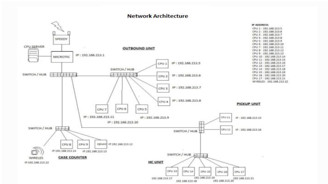
Figure 2. Network Topology
