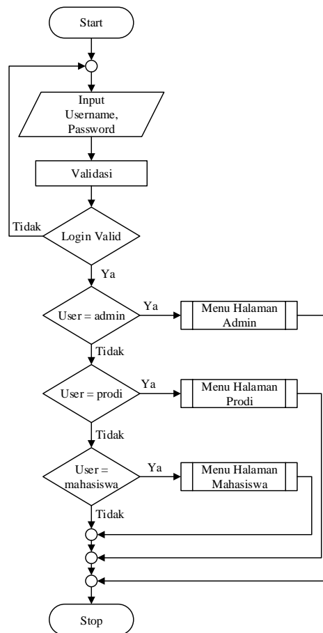
Gambar 5. Program Flowchart Login
