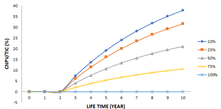
Fig. 4. Cumulative Net Present Value curve of tax variations.
