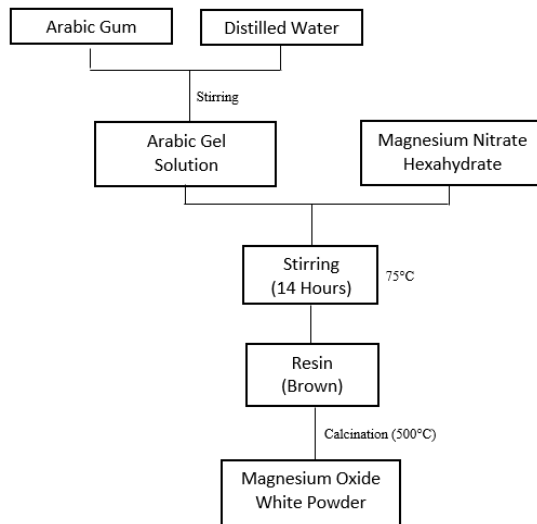
Fig. 1. Schematic of the sol-gel method of manufacturing magnesium oxide nanoparticles
