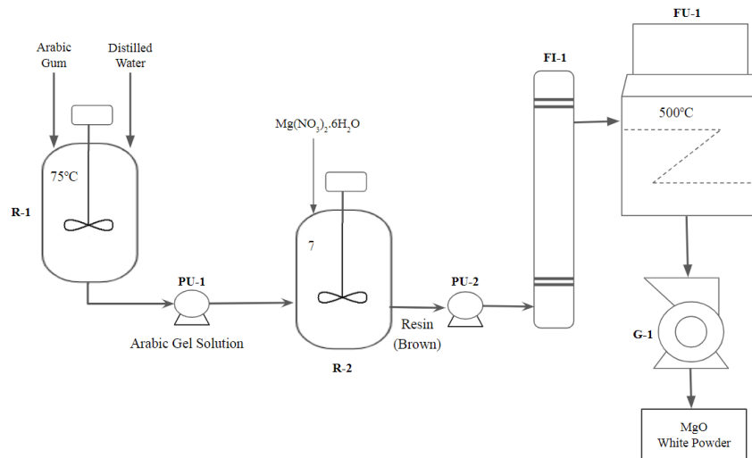
Fig. 2. Illustration of the flow diagram for the manufacture of magnesium oxide nanoparticles.
