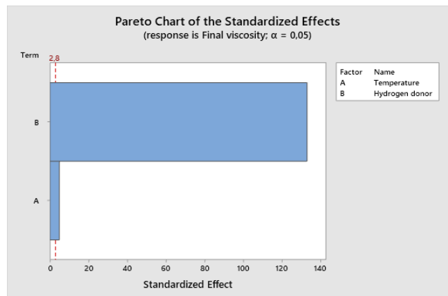
Figure 4. Pareto chart of standardized effects Source: Authors
