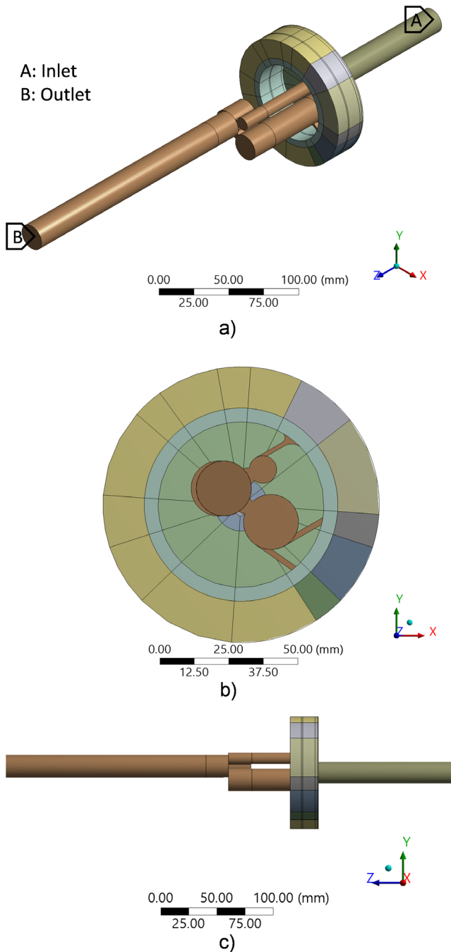
Figure 2. Volume of fluid extracted from the vortex reactor: a) isometric view with inlet and outlet domains, b) front view, c) side view Source: Authors
