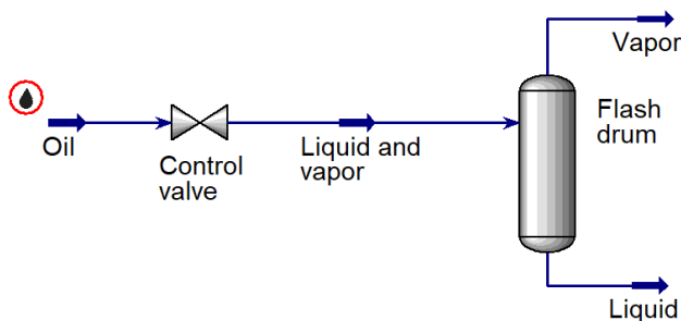
Figure 3. Aspen HYSYS configuration for oil characterization Source: Authors
