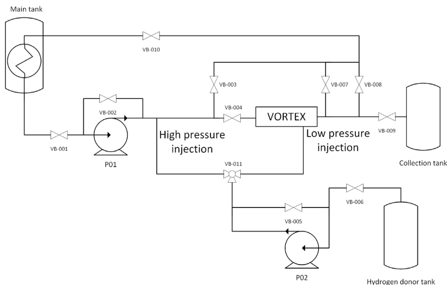
Figure 1. Diagram of the vortex reactor system Source: Authors
