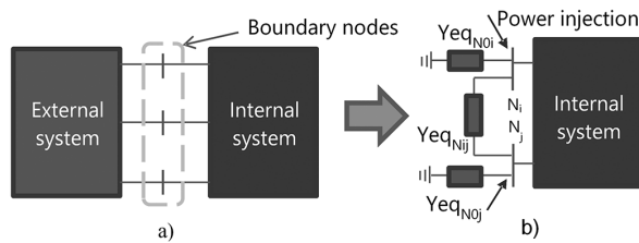
Figure 2. a. Power system division for reduction purpose. b. Equivalent network after Ward equivalent. Source: (Deckmann et al., 1980).
