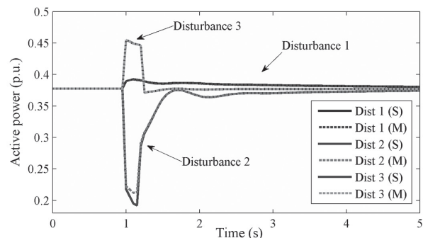
Figure 7. Active power response of load area equivalent under three different scenarios.
