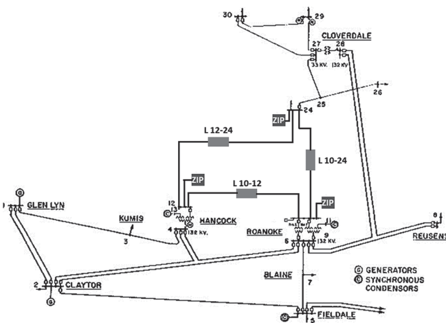
Figure 6. Equivalent power system for modified IEEE 30-bus system.
