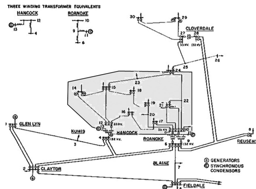
Figure 4. Test system division for reduction.
