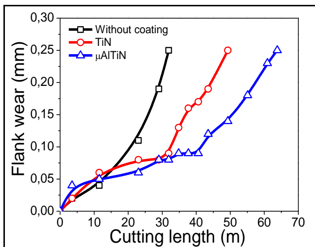
Figure 8. Curves for edge flank wear c_f the length of the cutting of different coatings used for the HSM of Ti6Al4V
