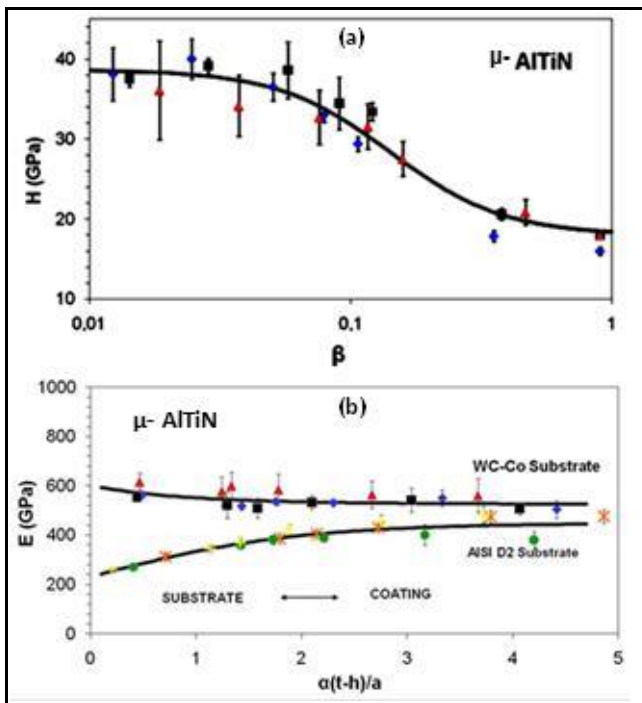
Figure 5. (a) hardness cf relative penetration depth ( \beta ) for the \mu -AlTiN coating on WC-Co substrate for different thicknesses, adjusted with Korsunsky's model (Korsunsky, 1998) and (b) comparison of Young's modulus for the \mu -AlTiN coating on AISI D2 steel and WC-Co substrate, adjusted with King's modified model (Saha et al. , 2002).
