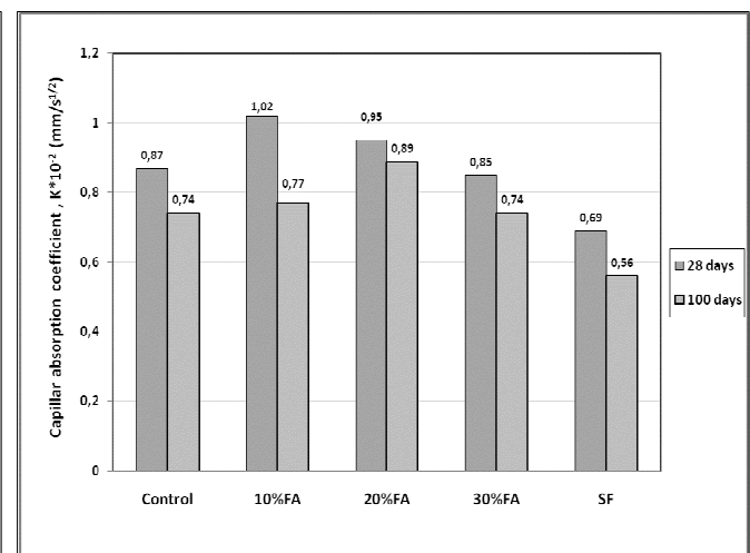
Figure 4. Capillary absorption coefficient
