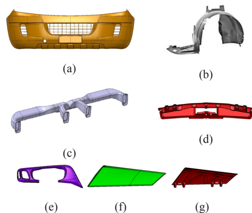
Figure 2. Sample figure of (a) bumper, (b) wheel arch, (c) air duct, (d) insert, (e) instrument panel frame, (f) glove compartment exterior and (G)glove compartment interior (Cagliano and Chiabert, 2018)
