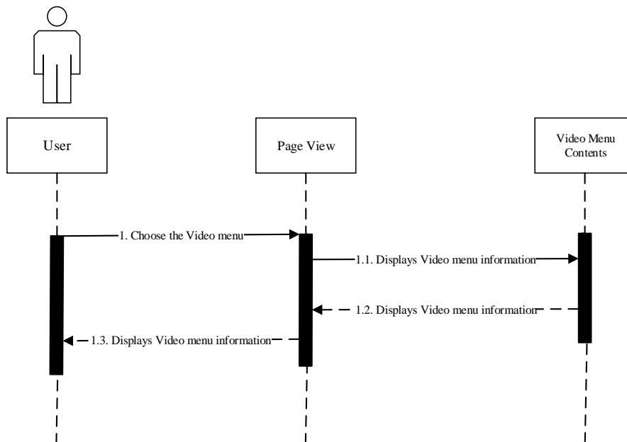
Figure 4. Sequence Diagram Video Menu.
