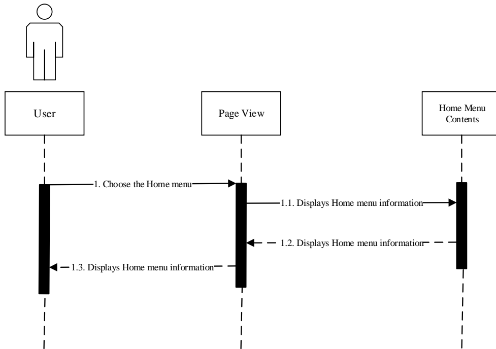
Figure 1. Sequence Diagram Home Menu.
