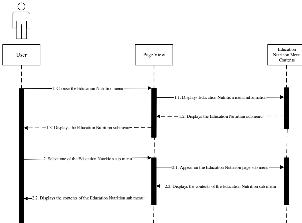
Figure 2. Sequence Diagram Education Nutrition Menu.
