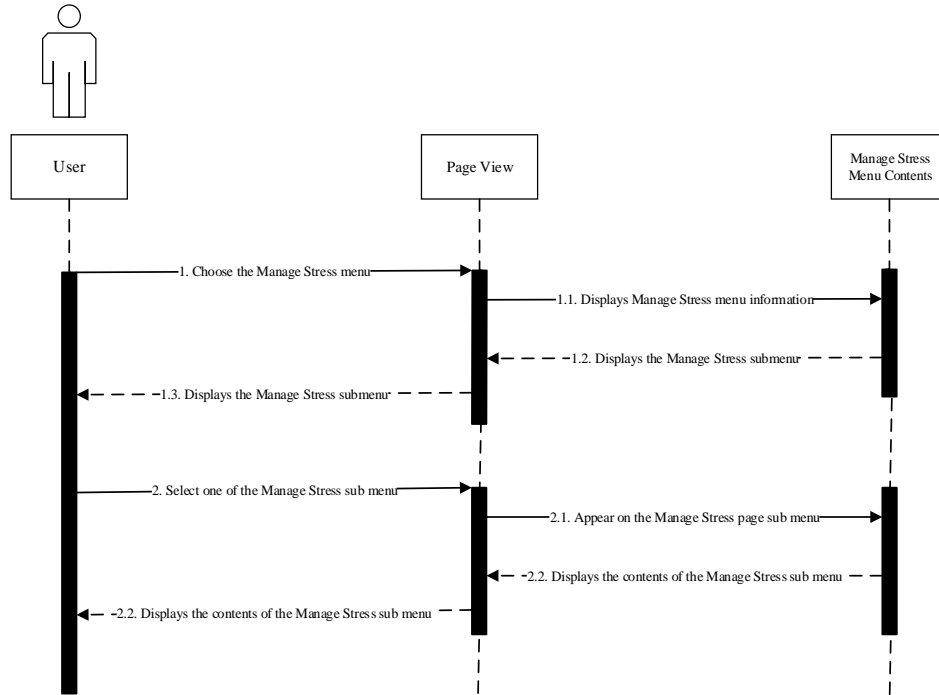
Figure 3. Sequence Diagram Manage Stress Menu.
