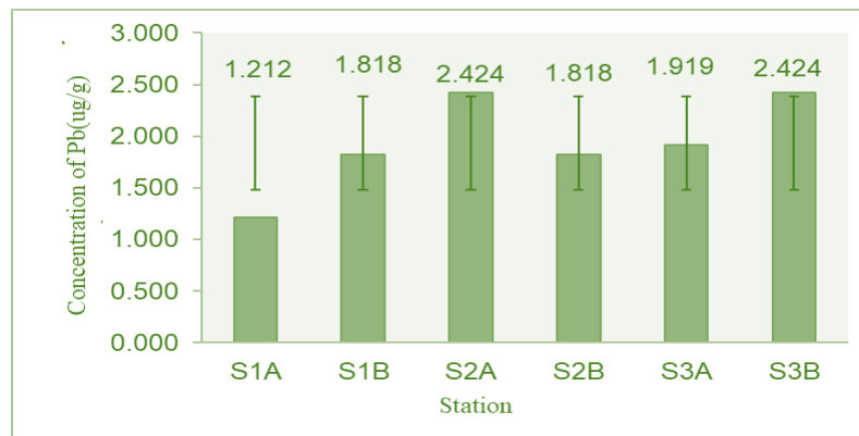
Figure 2. Heavy metal Pb concentration on green champa leaves in each station, i.e. S1 is station 1, S2 is station 2 and S3 is station 3; A is the upper leaf and B is the lower leaf.
