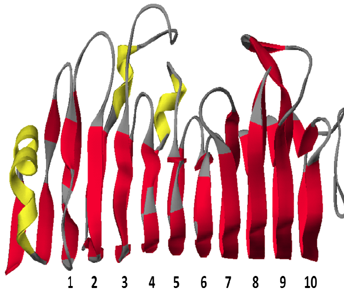
Fig. 2: Three dimensional structure of PGII-1CZF. Complete ten rung (number 1-10).
