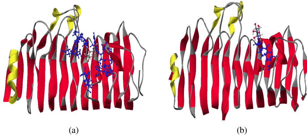
Fig. 3: Location of the ligand (GTR) in the structure; (a) GTR is docked in structure from Aspergillus niger (1CZF) (b) location of GTR in the structure from Stereum purpureum (1KCC).
