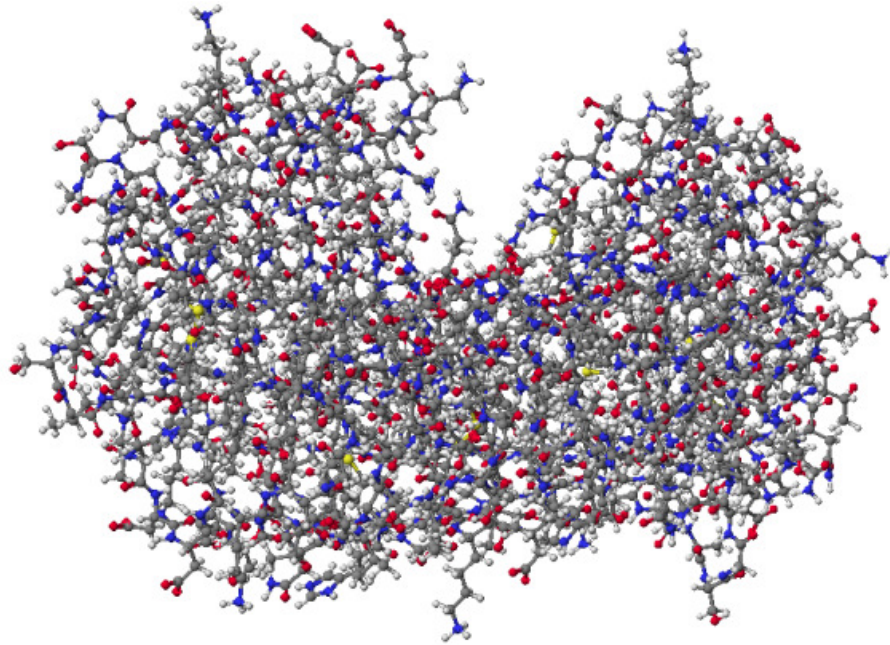
Fig. 1: Cleaned structure of polygalacturonase (PGII-1CZF).
