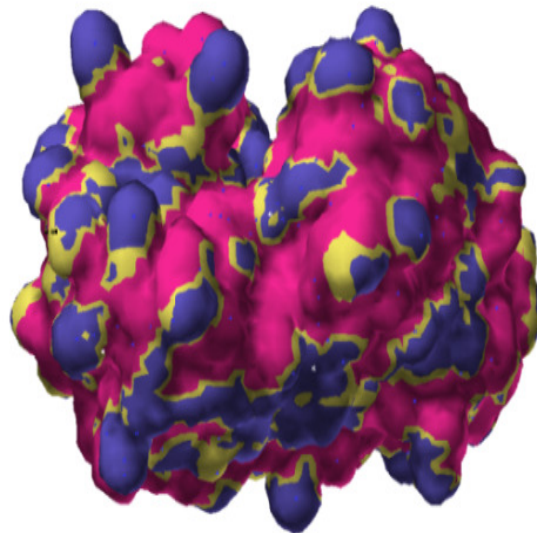
Fig. 4: Accessible surface of active site.
