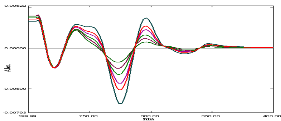
Figure No. (10): Second derivative spectra of mixtures containing of (4-20 \mu\text{g/mL} ) Ciprofloxacin hydrochloride and Mebeverine hydrochloride 8 \mu\text{g/mL}
