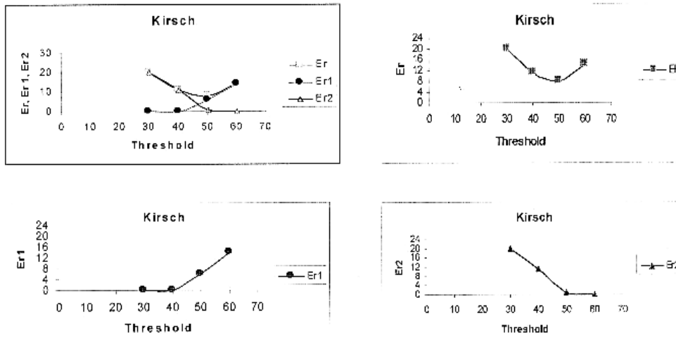
Figure (3) Relationship between (Er, Er1, &Er2) and Thresholds where the axis of (Er, Er1, Er2) multiply by 10 -3
