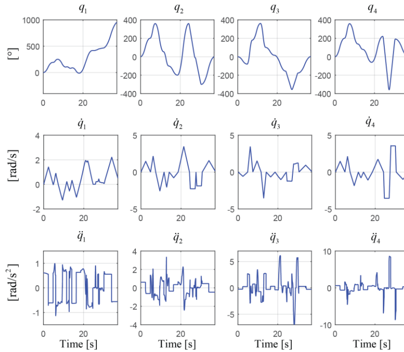
Fig. 2 Reference trajectories of the SDT joints
