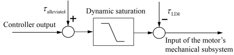
Fig. 3 Decoupling of the inverse dynamic model
