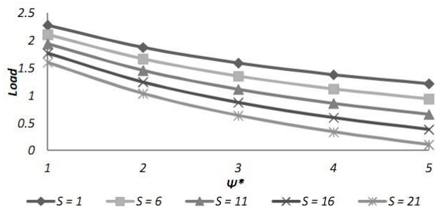
Fig. 27 Variation of load carrying capacity with respect to \psi^* and S
