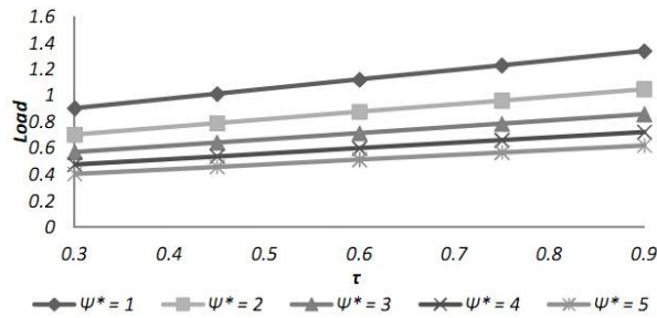
Fig. 19 Variation of load carrying capacity with respect to \tau and \psi^*
