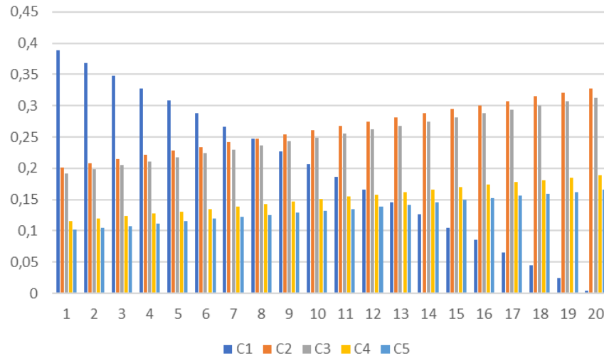
Fig. 2 Review of criteria weight coefficients changes
