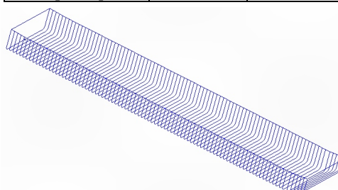
Fig.1. The hull-lines of the 23000 t barge (B40) [2].
