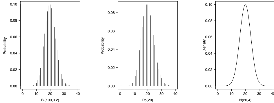
FIGURE 3: Graphical representation of the probability mass function of the Bi(100, 0.2) distribution and the Po(20) distribution, and probability density function of N(20, 4) distribution.
